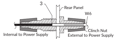
JF1 to JF4 detail (for fiber optic cable installation)
